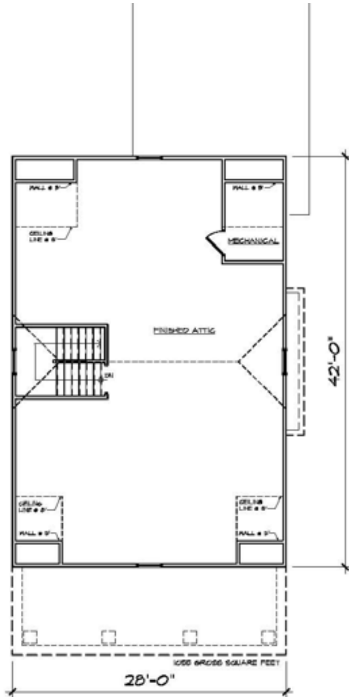
ATTIC FLOOR OPTION I 9/32"=1'-0"
